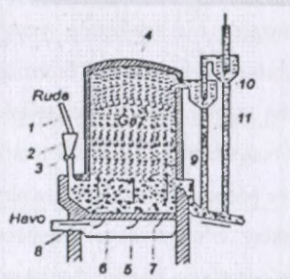
13.4-rasm. Mis rudalarini "qaynovchi qatlam" ostida boyitish qurilmasining sxemasi. 1-transportyor; 2-bunker; 3-dozator; 4-ish kamerasi; 5-havo kamerasi; 6-nasadka; 7-havo kiritish teshiklari; 8-havo kiritish teshigi; 9-kanal; 10-tsiklonlar; 11-trubalar.
