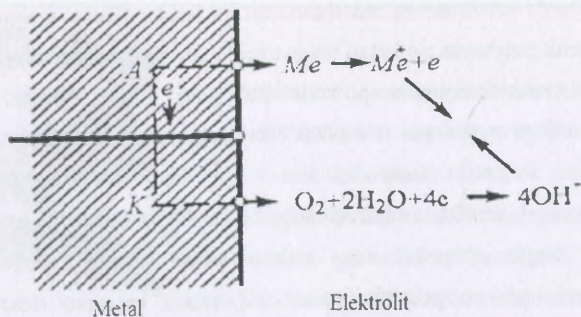
11.2-rasm. Korrozion element sxemasi
