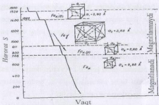
4.11-rasm. Haroratga qarab temirning kristallanishi
