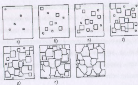
6.11-rasm. Metallarning kristallanish jarayonining sxemasi
