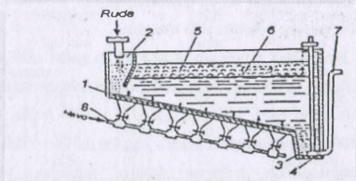
13.3-rasm. Mis rudalarni flotatsion boyitish mashinasining sxemasi; 1- rezinalangan to'qima; 2-kamera; 3-begona jinslarni to'plash chuquri; 5- ko'prik; 6-mis konsentrat olish teshigi; 7-suv trubasi; 8-truba(chapda).
