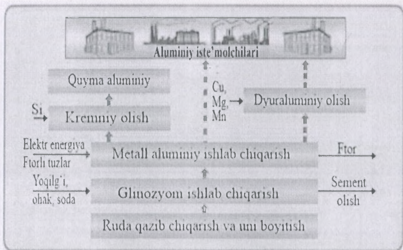
7-rasm. Aluminii ishlab chiqarish
