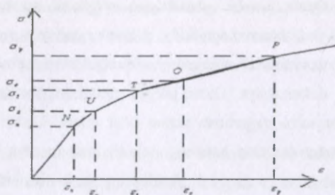
7.1-rasm. Nisbiy uzayishni deformatsiya \epsilon
