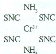
trans-izomer
