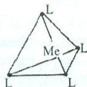
tetraedr
