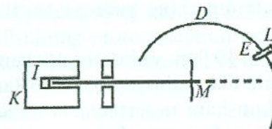
5- rasm. \alpha - zarrachalarning yupqa metallar pardadan o'tishi.
