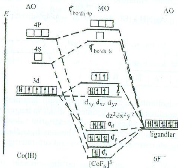
27 rasm. Molekular orbitallar usulida past spinli [\text{Co}(\text{NH}_3)_6]^{3+} va yuqori spinli [\text{CoF}_6]^{3-} komplekslarining energetik diagrammalari tuzilishi.
