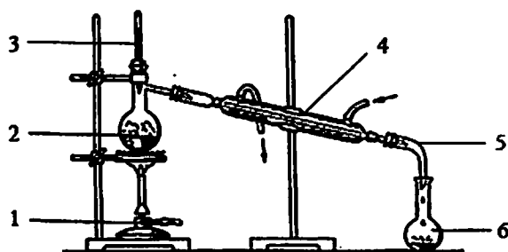
10-rasm. Atmosfera bosimida oddiy haydash asbobi:
