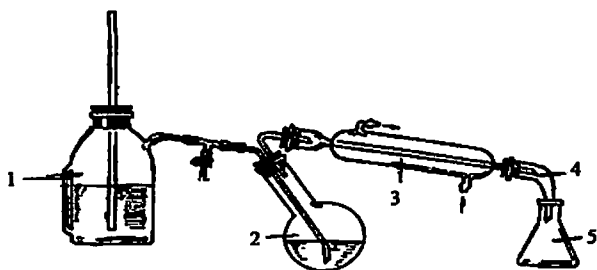
11-rasm. Suv bug'i bilan haydash asbobi:
