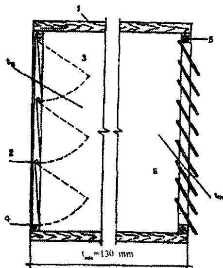
4.4.4-rasm. Ventilatsiyali klapan qurilmasi: 1-qobiq; 2-o'q; 3-sterjen; 4-klapan (jez, b=0.2 mm); 5-oldingi rom; 6-darpardalar.
