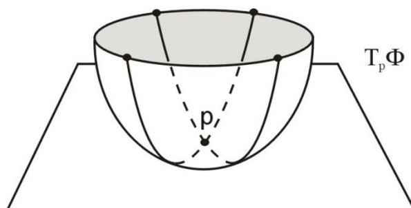
Elliptik nuqta
