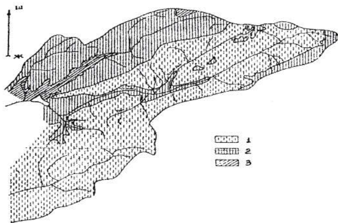
3.5.2-rasm. Tuproq yuvilishi kartasi, \text{t/km}^2 \times \text{yil} (Chirchiq – Ohangaron havzasi, O.P.Sheglova, 1983-y.) 1 – 100-200, 2 – 200-500, 3 – 500-1000
