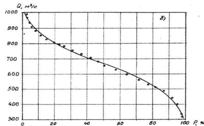
1.10.3-rasm. Daryo oqimining ta'minlanish (b) egri chizig'i.
