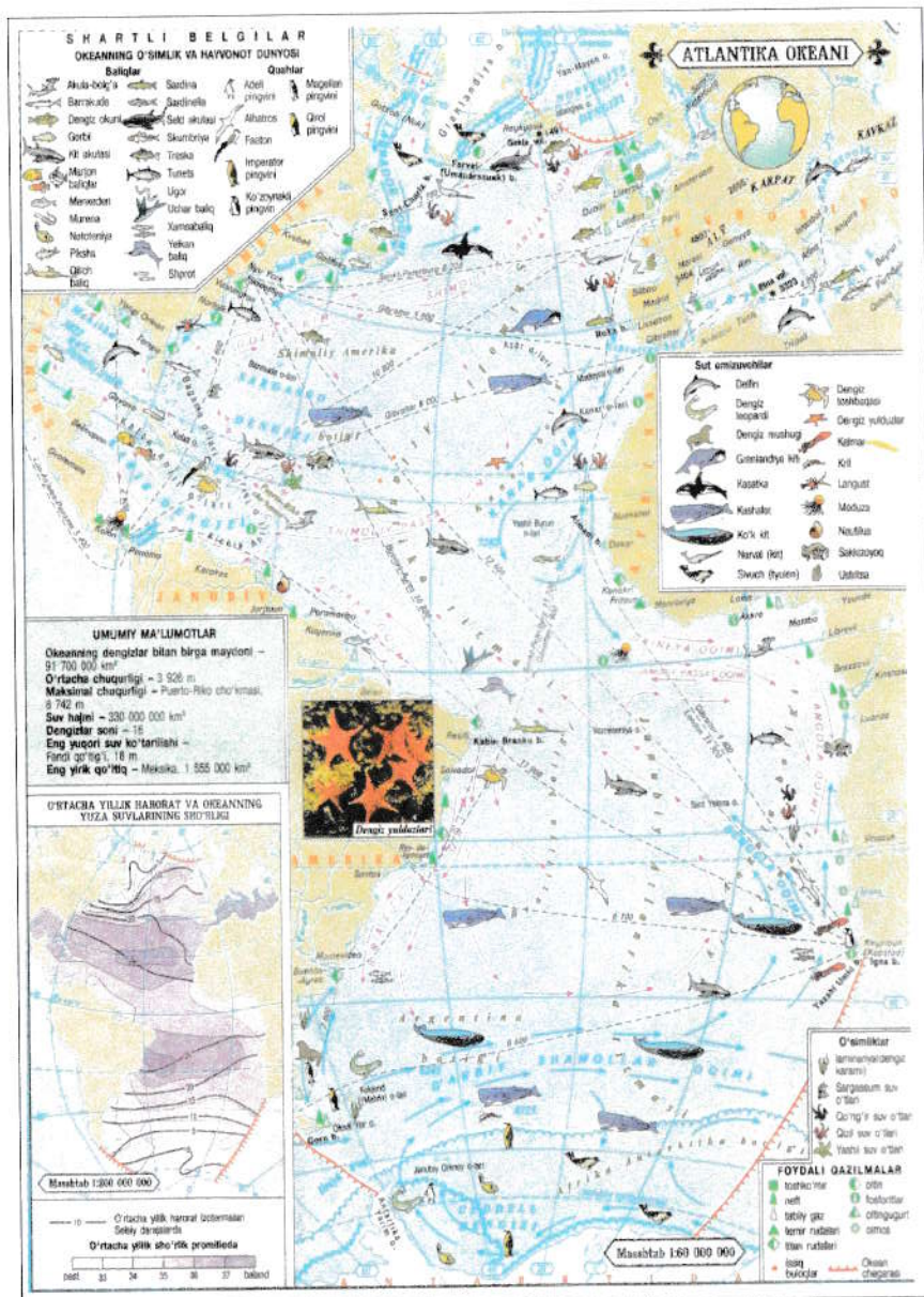
19-rasm. Atlantika okeani tabiiy kartasi
