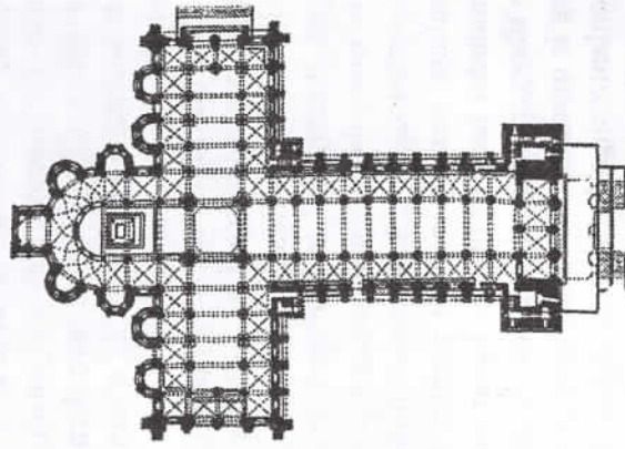
Rasm-84. Sant Yago de Compostela sobori tarxi. 1078 – 1128-yy.
