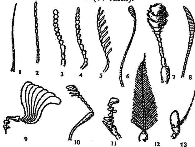
67-rasm. Hasharotlar mo'ylovi xillari: 1- qilsimon, 2-ipsimon, 3-cho'tkasimon yoki marjonsimon, 4-arrasimon, 5-taroqsimon, 6-to'g'nog'ichsimon, 7-cho'qmorsimon, 8-duksimon, 9-plastinka-to'g'nog'ichsimon, 10-taroq-tizzasimon, 11-noto'g'ri tizzasimon, 12-patsimon, 13-qildor.
