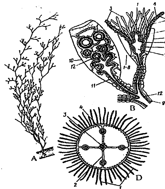
19-rasm. Dengiz gidroid polipi obeliya (Mavlonov, Xurramov, Norboyev, 2002)
