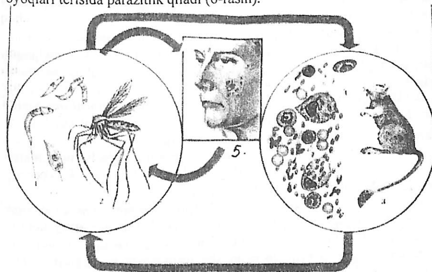
6-rasm. Teri leyshmaniyasi( Leishmania tropica )ning rivojlanish jarayoni:
