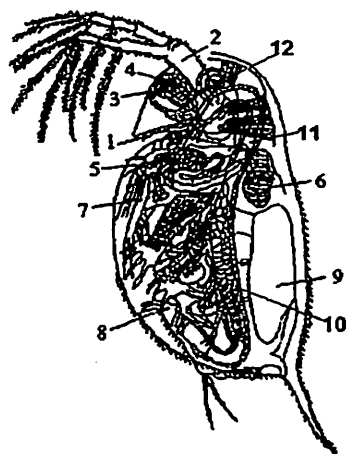
55-rasm. Dafniyaning tuzilishi: 1-antenullasi, 2-antennasi, 3-nauplius ko'zi, 4-murakkab ko'zi, 5-maksillyar bezi, 6-yuragi, 7-ko'krak oyoqlari, 8-ayricha, 9-nasl xonasi, 10-tuxumdoni, 11-muskullari, 12-jigar o'simtasi.
