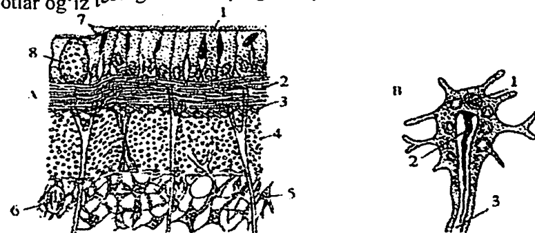
23-rasm. A-oq planariyaning teri-muskul xalta kesmasi: 1-teri epiteliysi, 2-halqali muskullar, 3-qiyshiq muskullar, 4-bo'ylama muskullar, 5-parenxima hujayralari, 6-rabdit hosil qiluvchi hujayralar, 7-rabditlar, 8-teri bezlari. B-ayirish sistemasini uchki hujayrasi: 1-yadro, 2-hilpillovchi kipriklar, 3- hujayra nayi.
