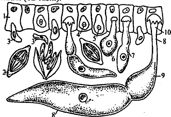
12-rasm. Gregarinalarning rivojlanishi: 1-ichak epiteliy hujayrasi; 2-spora; 3-sporozoitlar; 4-5-epiteliy hujayrasidagi sporozoitlar; 6-7-sporozoitning o'sib gregarinaga aylanishi; 8-deytomerit; 9-protomerit; 10-epimerit.
