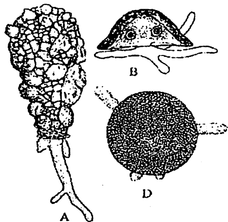
8-rasm. Chig'anoqli amyobalar: A-Diflyugiya, B-Arcella, D-Arcellaning orqa tomondan ko'rinishi
