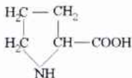
Prolin
