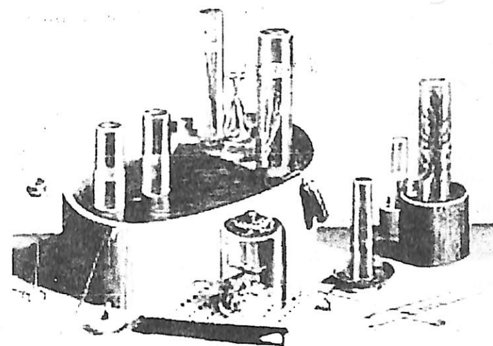
22-rasm. Pristlining gazlarni simob ustida yig'ish asbobi
