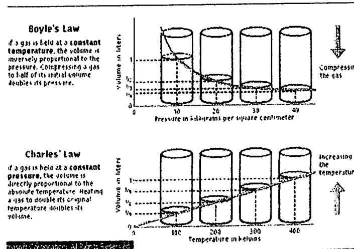
20-rasm. Boyle qonunining ko'rinishi
