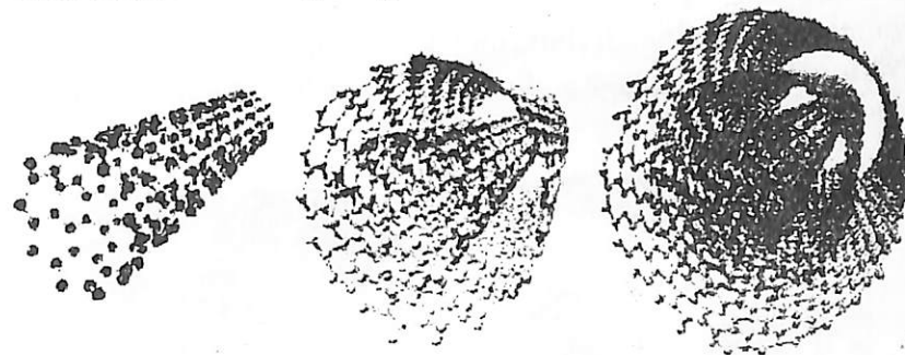
42-rasm. Nanotrubkalar
