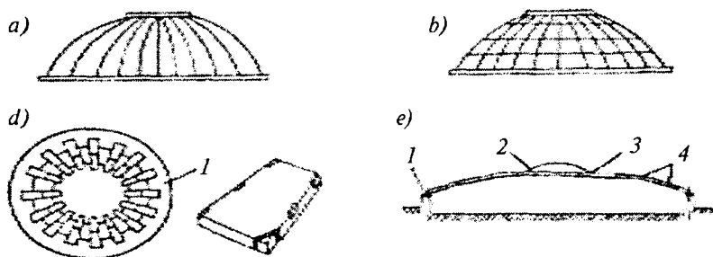
6.5- rasm. Yig'ma gumbazlar:
