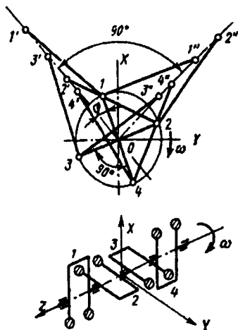
2.15-rasm. \gamma = 90^\circ bo'lgan V simon sakkiz silindrlı dvigatelning muvozanatlanganligini tahlili uchun.
