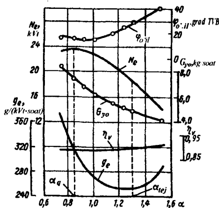
7.1-rasm. Drossel to'sma qopqoqning o'zgarmas holatida ( \eta_v = const ) aralashma tarkibi bo'yicha rostdlash tavsifi \varphi_{op} = 100\% , n = 2000 \text{ min}^{-1} .
