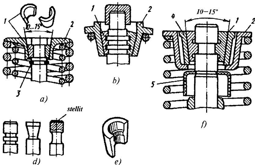
9.12-rasm. Klapan prujinasining mahkamlash elementlari (a, b, d, e, f).
