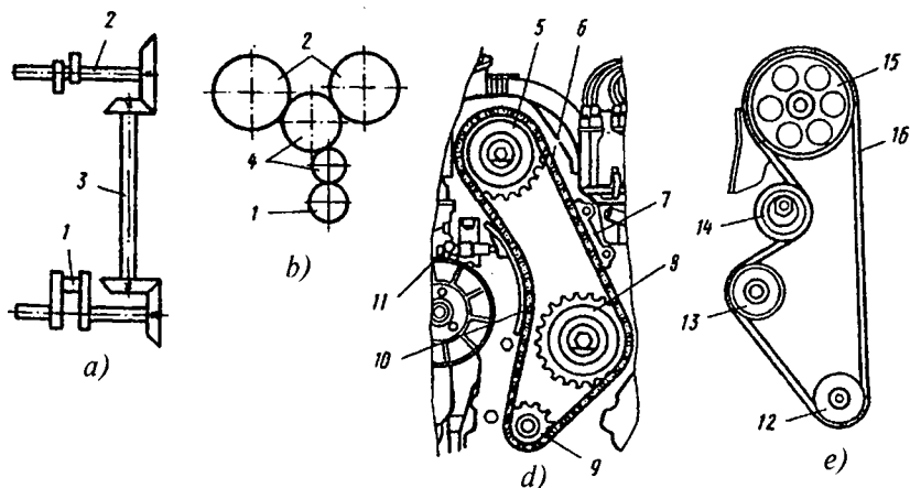
9.8-rasm. Yuqori taqsimlash vallariga yuritma (a...g):
