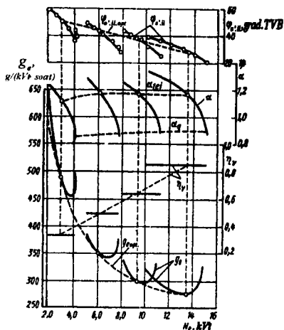
7.3-rasm. Eng maqbul rostlash tavsifi: iV_h = 1,1 , n = 2000 \text{ min}^{-1}
