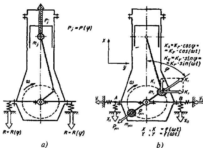
1.8-rasm. Dvigatel tayanchiga inersiya kuchining ta'siri:
