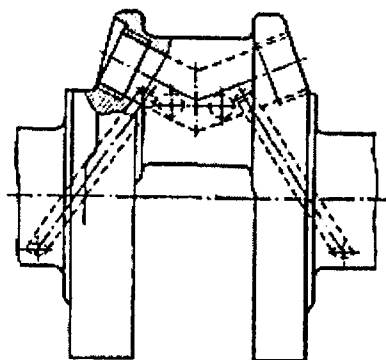
7.5-rasm. Shatun podshipniklariga moy keltirish.
