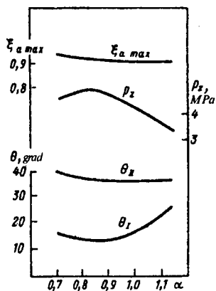
3.24-rasm. Yonish jarayoni fazalarini davomiyligiga \alpha ning ta'siri ( \varepsilon = 8,9 ; n = 3000 \text{ min}^{-1} ; drossel to'liq ochiq).
