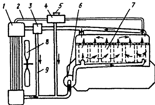
11.1-rasm. Suyuqlik bilan sovitiladigan tizimning prinsipial sxemasi: 1 – radiator; 2 – bug'-havo naychasi; 3 – termostat; 4 – kengayish baki; 5 – kengayish bakining tiqini; 6 – nasos; 7 – silindrlar blokining g'ilofi; 8 – ventilator; 9 – aylanib o'tuvchi naycha.
