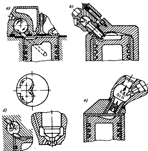
3.39-rasm. Ajratilgan yonish kameralari:
