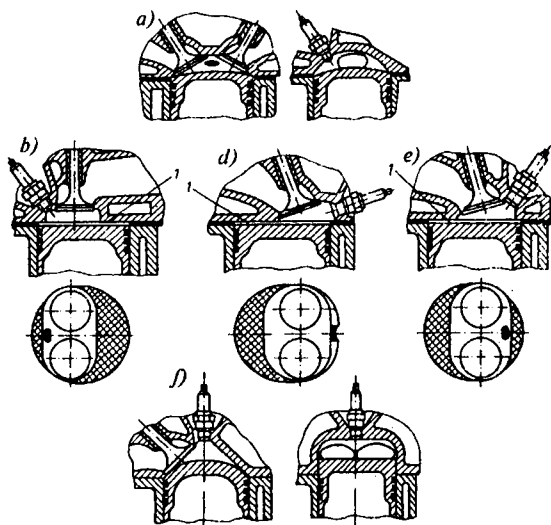
3.25-rasm. Uchqundan o't oldiriladigan dvigatellar yonish kameralarining sxemasi: a — yarim doira; b — tekis ovalli; d — ponasimon; e — yarim ponasimon; f — chodirsimon; 1 — siqib chiqaruvchi.
