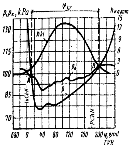
3.4-rasm. To'rt taktili dvigatelnining kiritish jarayoni-da p va p_k larning o'zgarishi: \varphi_{kir} — kiritish fazasi.
