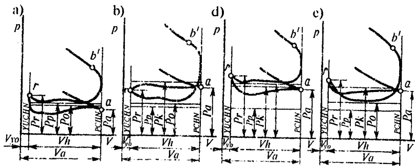
3.1-rasm. To'rt taktli dvigatelning gaz almashinuvi diagrammasi:
