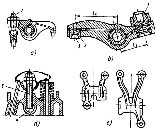
9.18-rasm. Koromislolar ( a, b, d, e ).
