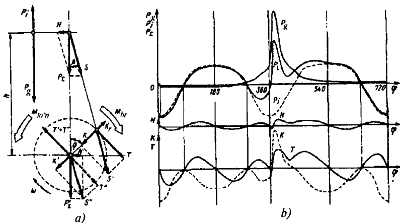
1.9-rasm. KSHM dagi kuchlar:
