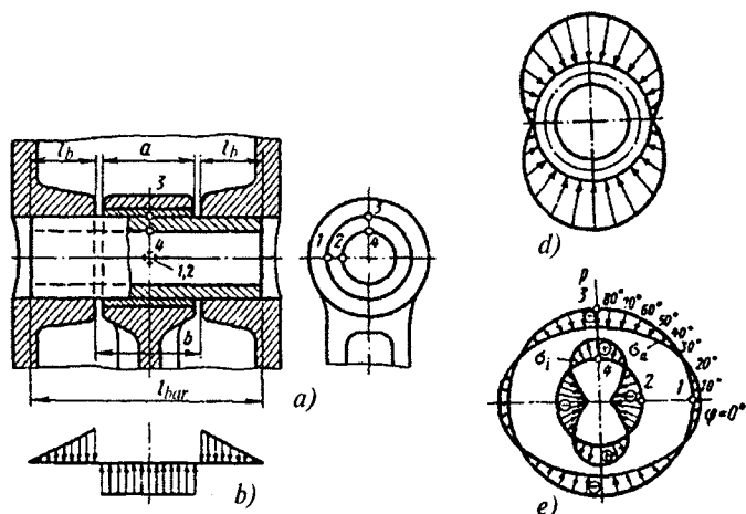
5.20-rasm. Porshen barmog'ini hisoblash:
