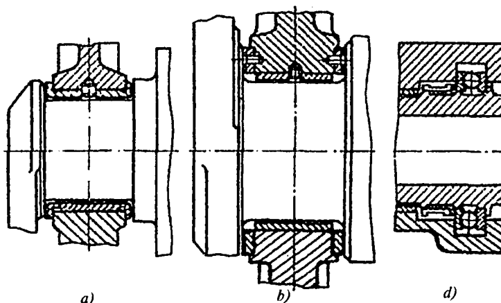
7.8-rasm. Tirsakli valning tirak podshipniklari:
