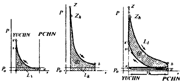
1.8-rasm. Siklning indikator ishini aniqlash.
