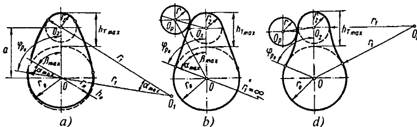
9.22-rasm. Kulachoklarning profillari: a – qavariq; b – tangensial; d – botiq.
