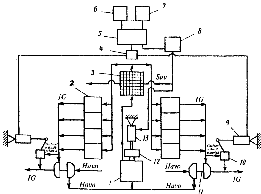
7.16-rasm. Boshqariladigan kombinirlangan (bosim ostida kiritish)
