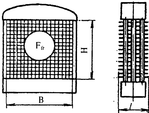
11.15-rasm. Radiatorni sovitish panjarasining gabarit o'lchamlari: B – kengligi;
