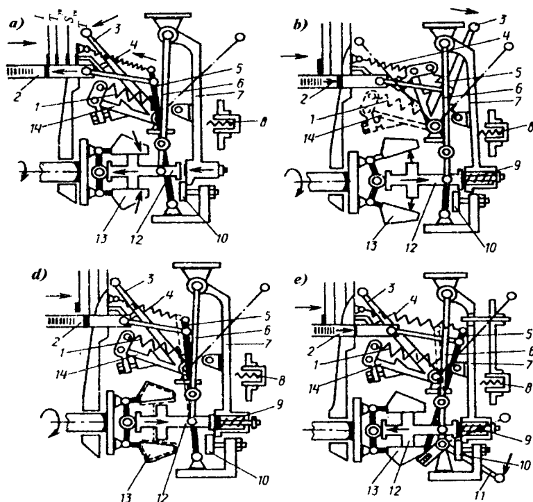
5.41-rasm. Barcha rejimli rostlagich ishlash sxemasi: a — ishga tushirish rejimi; b — salt yurish rejimi; d — nominal rejim, tuzatishning boshlanishi; e — maxsus richag orqali to'xtatish rejimi; 1 — ishga tushirish; TYU — to'liq yuklama; SYU — salt yurish; T — to'xtash.
