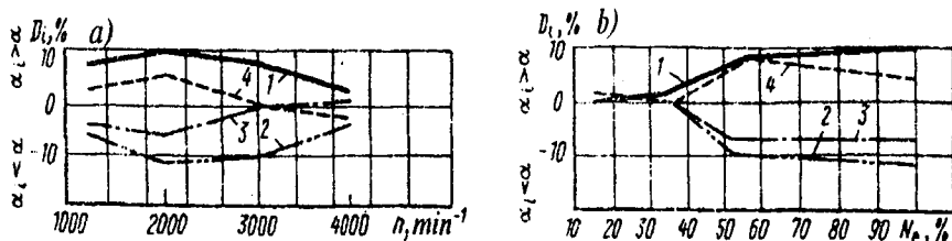
3.18-rasm. To'rt silindrli karbyuratorli dvigatelda quyidagilarga bog'liq holda aralashma tarkibining notekislik darajasining o'zgarishi:
