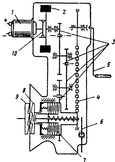
14.2-rasm. Inersion startyorning sxemasi.
