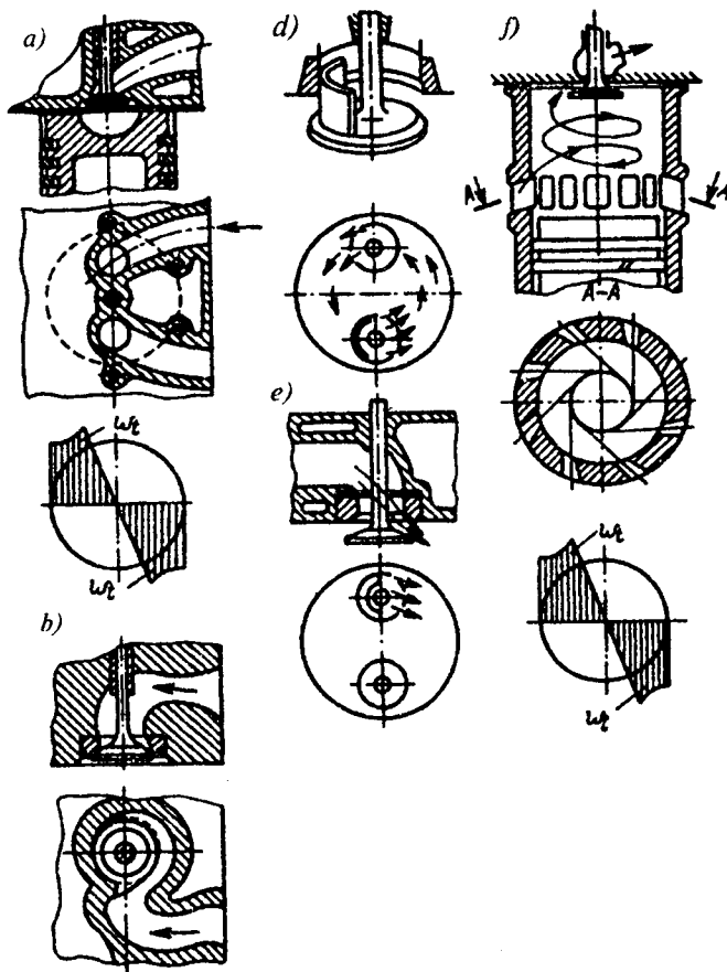
3.35-rasm. Kiritish jarayonida silindrda zaryadni aylanma harakatini hosil qilish usulini tushuntiruvchi tasvir sxemasi:
