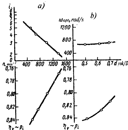
4.4-rasm. Siqish jarayoni oxiridagi zaryad harakatining eng optimal burchak tezligi \omega_{opt} ni to'ldirish koeffitsiyenti \eta_v , to'zitish teshiklari soni i_c (a) va yonish kamerasining nisbiy diametri d_{yo.k.} / D bilan o'zaro bog'liqligi (b).
