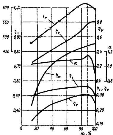
7.9-rasm. Karbyuratorli dvigatel ko'rsatkichlarining yuklama tavsifi bo'yicha o'zgarishi: n = 2000 \text{ min}^{-1} \epsilon = 7 ; iV_h = 6,0 \text{ l} .
