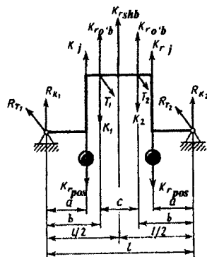
7.12-rasm. V simon dvigatel krivoshipining yuklanish sxemasi.
