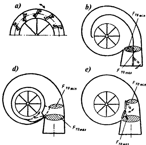
5.34-rasm. Turbinaning ichki rostlash usuli:
