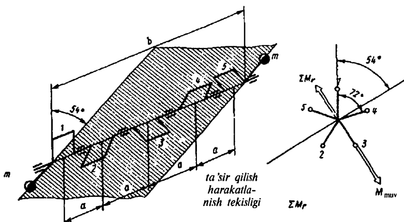
2.9-rasm. Burchagi \delta = 72^\circ bo'lgan besh krivoshipli tirsakli valni muvozanatlash.
