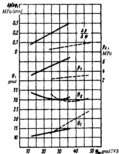
3.23-rasm. Yonish jarayoni fazalarining davomiyligiga \varphi_{o'it} ning ta'siri
