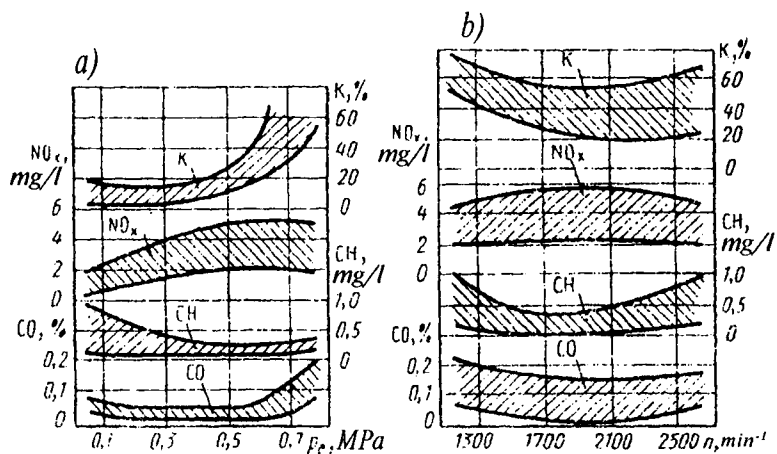
6.14-rasm. To'rt taktli dizellar IG ning zaharliligiga yuklama (a) va aylanishlar chastotasining (b) ta'siri.
