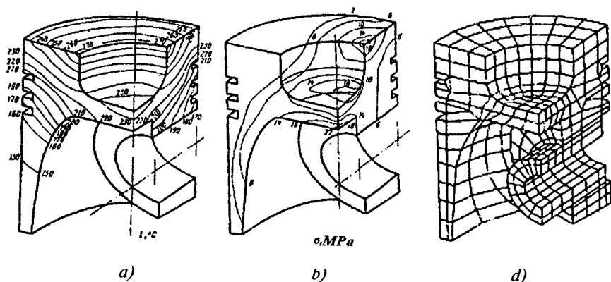
5.4-rasm. So'nggi element modeli (d) yordamida olingan dizel porshenining harorat maydoni (a) va eng kichik asosiy kuchlanishi (b).
