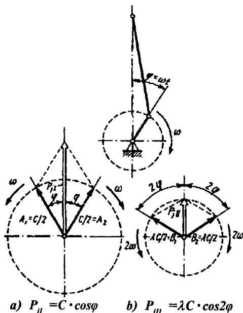
2.11-rasm. Inersiya kuch P_{II} (a) va P_{III} (b) larni grafikda aniqlash.
