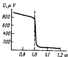
6.9-rasm. Kislorod datchik tavsifi ( \lambda — zond).
