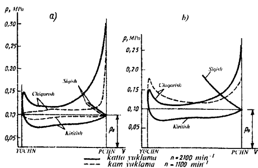
4.6-rasm. Turli aylanishlar chastotasida (a) va yuklamalarda (b) bosimsiz kiritiladigan dizel nasos yo'lining diagrammalari.
