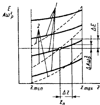
5.43-rasm. Regulator prujinasining dastlabki tortilishi va burchak tezligining turli qiymatlarida mexanikaviy sezgir element tavsifi:
