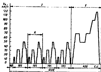
6.5-rasm. Yugurish borabanli stendda sinash rejimlari.
