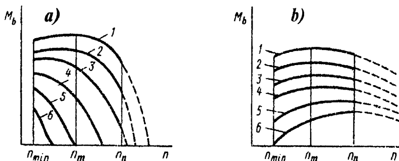
5.38-rasm. Tezlik tavsiflari: a — drossel to'smaqopqoqni turlicha ochilish miqdorida uchqundan o't oldiriladigan dvigatel: Dr_1 > Dr_2 > Dr_3 > Dr_4 > Dr_5 > Dr_6 ; b — plunjer faol yo'lining turli miqdorida dizel ( h_{faol} ): h_{faol1} > h_{faol2} > h_{faol3} > h_{faol4} > h_{faol5} > h_{faol6} .
