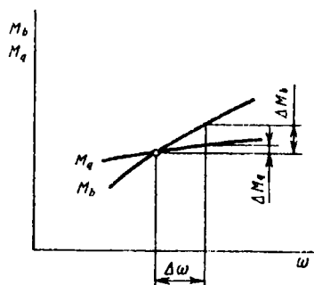
5.37-rasm. Dvigatelnig barqarorlik omilini aniqlash.
