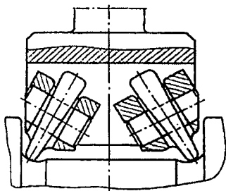
7.13-rasm. Galtellarga rolik bilan ishlov berish.
