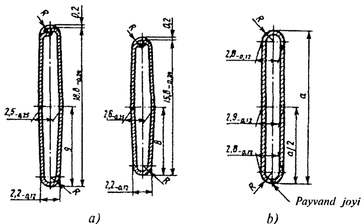
11.5-rasm. Radiator naychalari:
