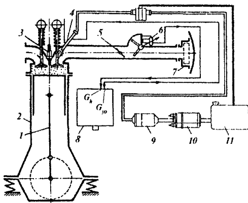
1.4-rasm. Kiritish tizimiga benzin purkaladigan dvigatelning sxemasi:
