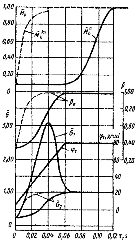
7.20-rasm. Drossel to'smaqopqoq tez
