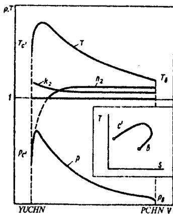
3.44-rasm. Kengayish jarayonida T , p , S , n_2 va k_2 larning o'zgarishi.
