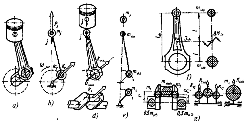
1.7-rasm. KSHM ikki massali dinamikaviy modelini tashkil qilish: a – KSHM; b – KSHM modeli; d – KSHM dagi kuchlar; e – KSHM massalari; f – shatun massalari; g – krivoship massalari.
