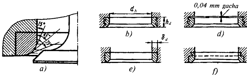
9.13-rasm. Klapanlar o'rindig'i (a...f).
