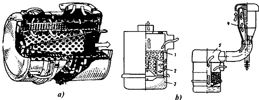
12.1-rasm. Tozalovchi elementi kartonli havo tozalagich (a) va kombinirlangan ikki bosqichli havo tozalagichlar (b): 1 – to'g'ri oqimli monotsiklon; 2 – kartonli toza'lovchi element; 3 – ajratilgan changni yig'ish uchun bunker; 4 – konussimon inersion panjara; 5 – inersion-moyli havo tozalagich.
