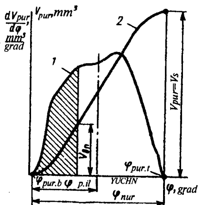
3.27-rasm. Purkashning differensial (1) va integral (2) tavsiflari.
