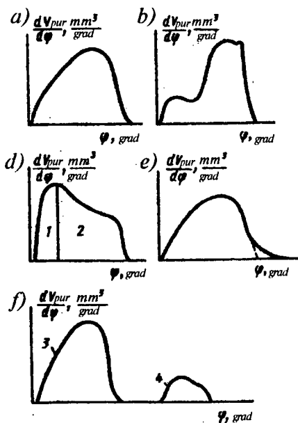
3.28-rasm. Purkashning differensial tavsiflarining turli (a....d) ko'rinishi.
