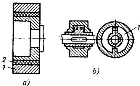
8.11-rasm. Buralma tebranishlar so'ndirgichlari sxemasi: a —molekular ishqalanishli ( I -inersion element, 2—elastik element); b —suyuq ishqalanishli ( I -suyuq to'ldirgich — silikon).
