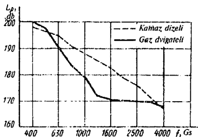
6.21-rasm. n = 2200 \text{ min}^{-1} bo'lganda KamAZ dvigateli indikator diagrammalarining spektrlari.
