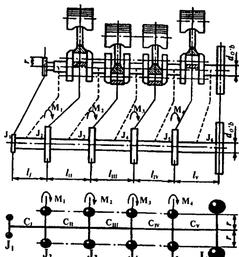
8.2-rasm. To'rt silindrli qatorli dvigatelning ekvivalent buralma tizimi.
