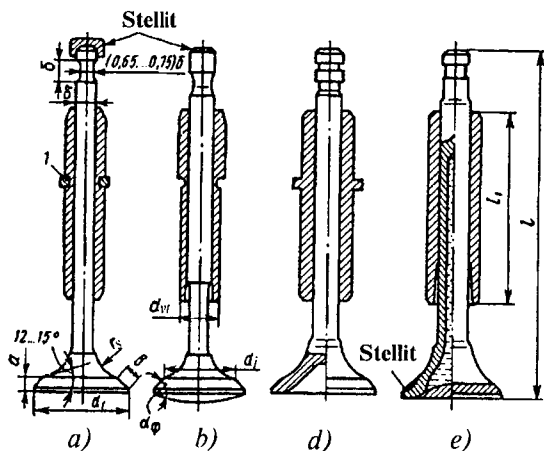
9.11-rasm. Dvigatellarning klapanlari: a, e-yassi; b-qavariq; d-lolasimon.
