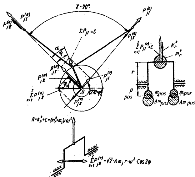
2.14-rasm. \gamma = 90^\circ bo'lgan ikki silindrlı V simon dvigatelni muvozanatlash.
