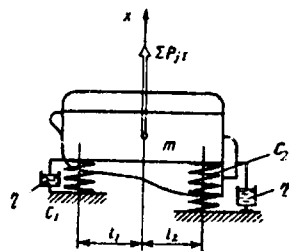
2.21-rasm. P_{ji} kuch ta'siridan osmada dvigatel tebranishini hisoblash sxemasi.
