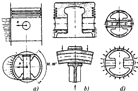
5.8-rasm. Porshenning deformatsiyalanishi:
