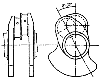
7.4-rasm. Siljilgan shatun bo'yinli krivoship.
