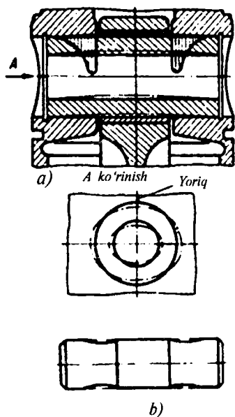
5.13-rasm. Porshen bobishkasining yuklamasi va deformatsiyasi: a—porshen bobishkalarida deformatsiya va kuchlanish; b—porshen barmog'ini profillash.
