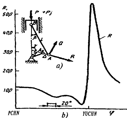
1.15-rasm. Shatun podshipnikdagi tirqish \Delta ni hisobga olinishidagi sxemasi (a) va tirsakli valning burilish burchagiga dinamikaviy reaksiya R ning bog'liqlik grafigi (b); A — yuklamaning keskin oshish qismi.
