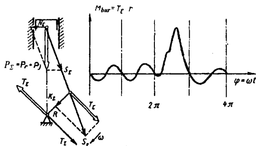
8.12-rasm. K_r kuch ta'siridan krivoshipning egilish tebranishlari paydo bo'lishi.
