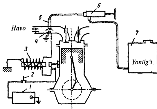
14.4-rasm. Havoni isitish sxemasi:
