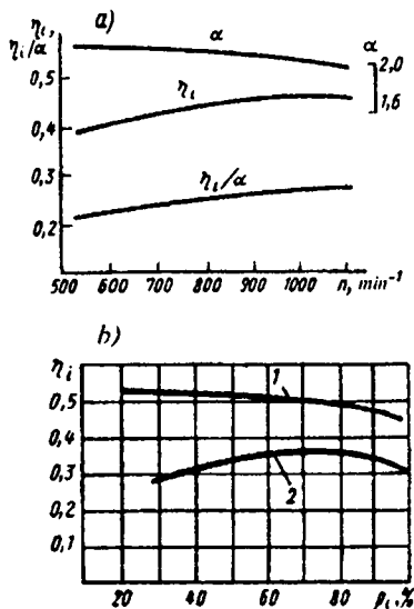
4.5-rasm. \eta_i , \eta_i/\alpha va \alpha larning aylanishlar chastotasiga (a) va \eta_i ning yuklamaga (b) bog'liqligi:
