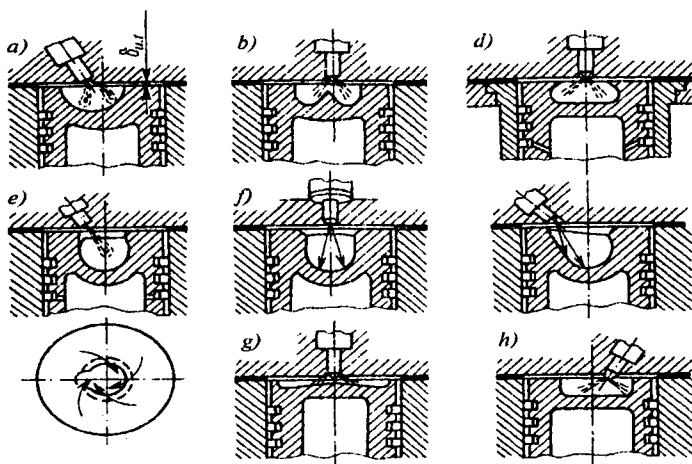
3.34-rasm. Porshendagi yonish kameralar:
