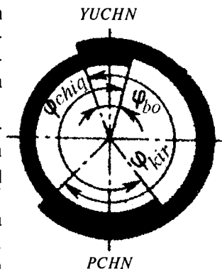
3.3-rasm. To'rt taktli dvigatelning gaz taqsimlash fazasining diagrammasi.
