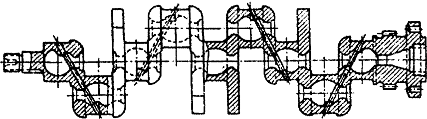
7.2-rasm. Cho'yandan tayyorlangan tirsakli val.
