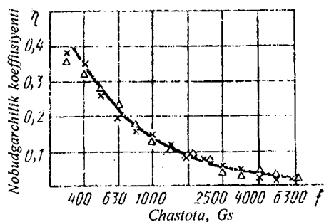
6.19-rasm. Dvigatel konstruksiyasidagi nobudgarchilik koeffitsiyentining chastotaga bog'liqligi: x-4CH 7,6/8 (VAZ-341) dvigateli; \Delta -4CH 8,2/7 (AZLK) dvigateli; — — — approssimirovchi egri chiziq.
