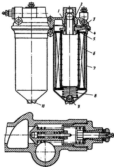
10.11-rasm. YAMZ-840 dvigatelining to'liq oqimli moy tozalash filtri:
