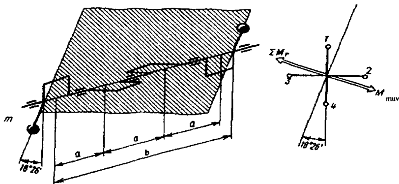
2.10-rasm. Krest shaklidagi tirsakli valni muvozanatlash.
