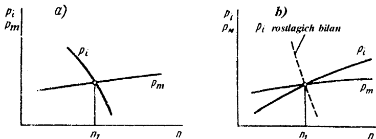
5.36-rasm. Salt yurish rejimlarining barqarorligi: a — barqaror; b — beqaror (rostlagichsiz).
