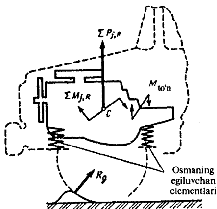
2.19-rasm. Osmada dvigatelning tebranishini keltirib chiqaradigan kuch omillari.
