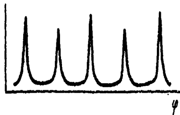
3.22-rasm. Ketma-ket sikllarning nobarqarorligi ( \varepsilon = 6,2 ; n = 1500 \text{ min}^{-1} ; \alpha = 1,23 ; drossel to'liq ochiq).
