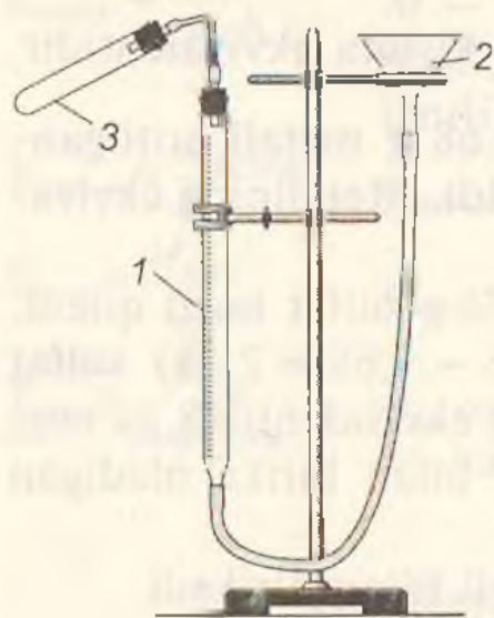
20-rasm. Ekvivalent aniqlanadigan asbob:
