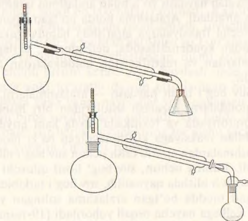
17-rasm. Oddiy sharoitda haydash.
