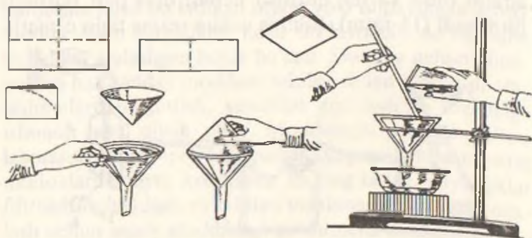
12-rasm. Filtr tayyorlash.
