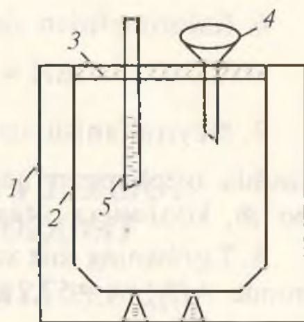
25-rasm. Kalorimetr:
