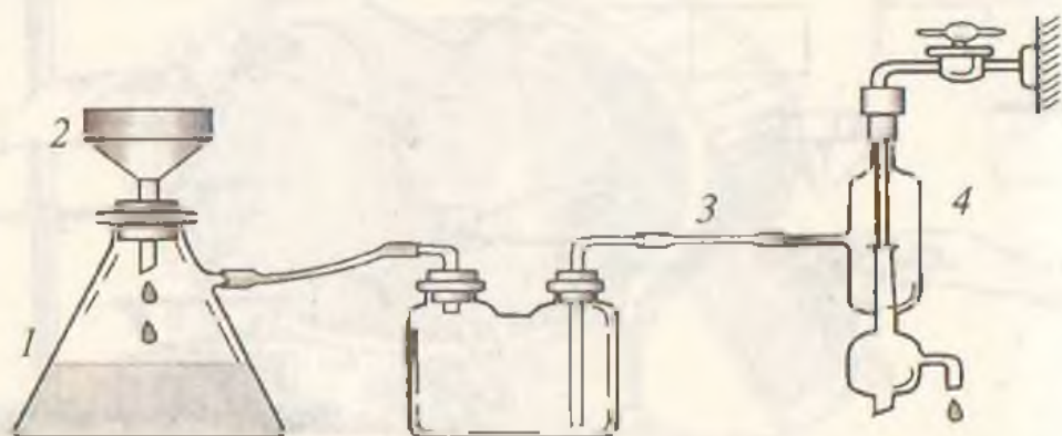
14-rasm. Past bosimda filtrlash.
