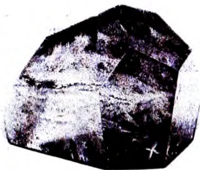
2- rasm. Morion.
