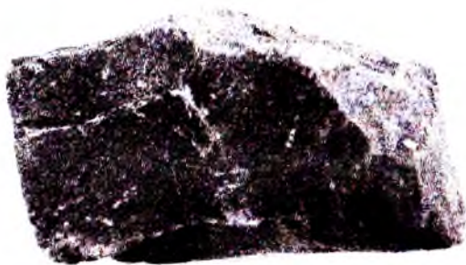
41- rasm. Dunit.
