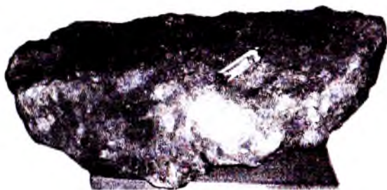
16- rasm. Fluorit.
